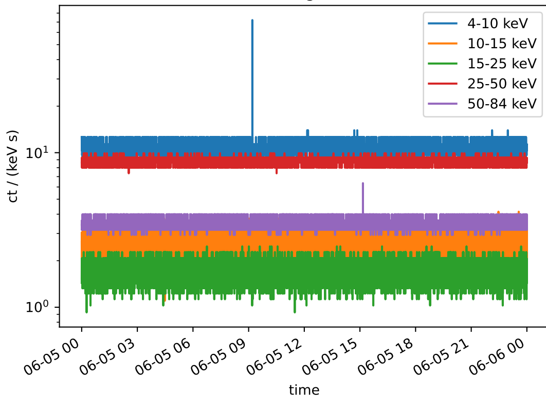
STIX QL Light Curve
